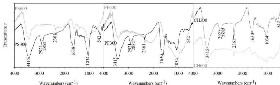
Figure 2-2. FTIR spectra of the biochars studied. PS: pineapple stubble; PF: oil palm fiber; CH: coffee hulls. Number after symbol indicates temperature of pyrolysis in ^{\circ}\text{C} .
