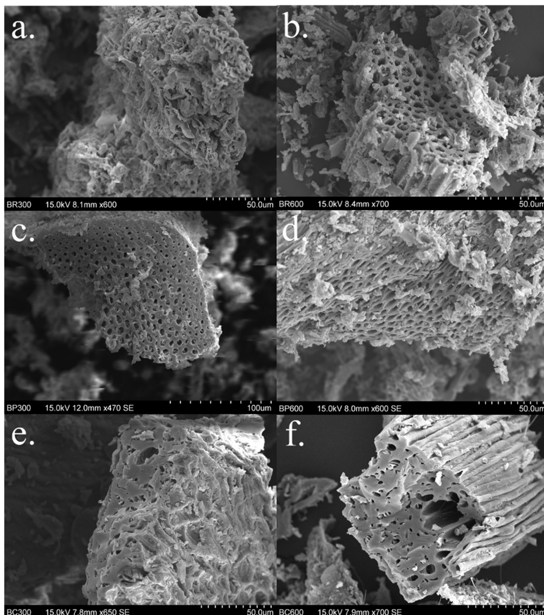
Figure 2-3. SEM images of biochars studied. a: PS300; b: PS600; c: PF300; d: PF600; e: CH300; f: CH600.
