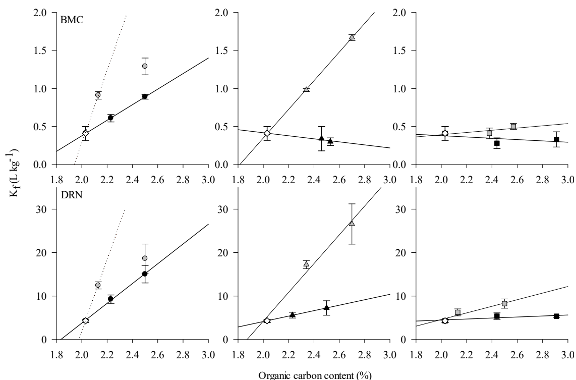
Figure 3-1. Distribution of K_f values of the pesticides bromacil (BMC, top) and diuron (DRN, bottom) as function of the total organic carbon content (TOC) in amended soil. Grey (◻) and black (◼) symbols correspond to materials charred at 300 °C and 600 °C, respectively. Circle represents pineapple stubble (○/●, PS), triangle palm fiber (△/▲, PF), and square coffee hull (◻/■, CH). White diamond (◇) corresponds to the values in control soil. Error bars correspond to standard deviation of three replicates. Dotted lines indicate an estimation of the expected linearity.
