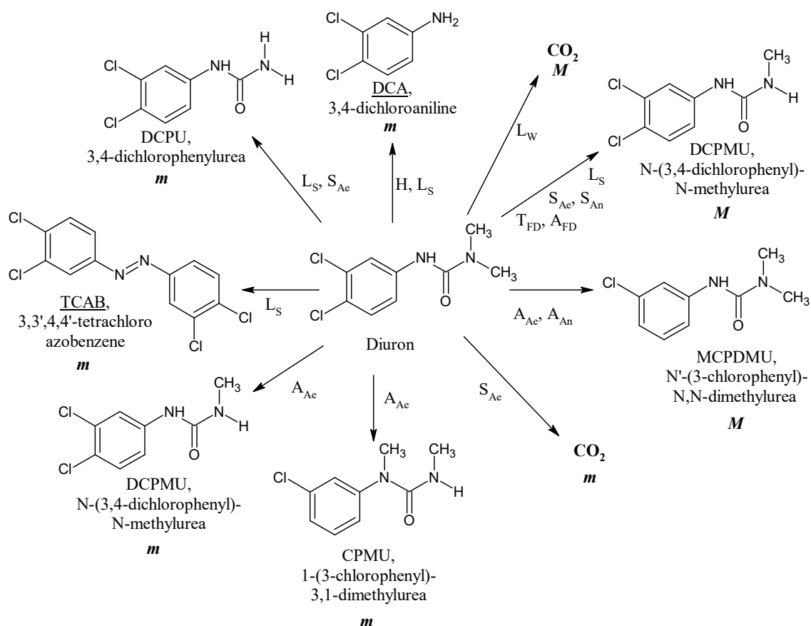
Figure 1-3. Transformation products and metabolites of DRN. Routes of transformation are codified as H (hydrolysis), L w (photodegradation in water), L s (photodegradation in soil), S Ae (aerobic soil metabolism), S An (anaerobic soil metabolism), A Ae (aerobic aquatic metabolism), A An (anaerobic aquatic metabolism), T FD (terrestrial field dissipation), A FD (aquatic field dissipation). M indicates major and m indicates minor metabolite. Underlined name indicates products of human health concern (Tixier et al., 2001; U.S. EPA, 2003).
