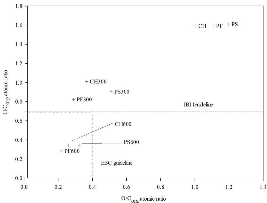
Figure 2-1. Van Krevelen diagram including the biochars and the corresponding feedstocks. Dotted line represents EBC criteria (EBC, 2012) and dashed line represents IBI criteria (IBI, 2015) to classify a charred material as biochar.
